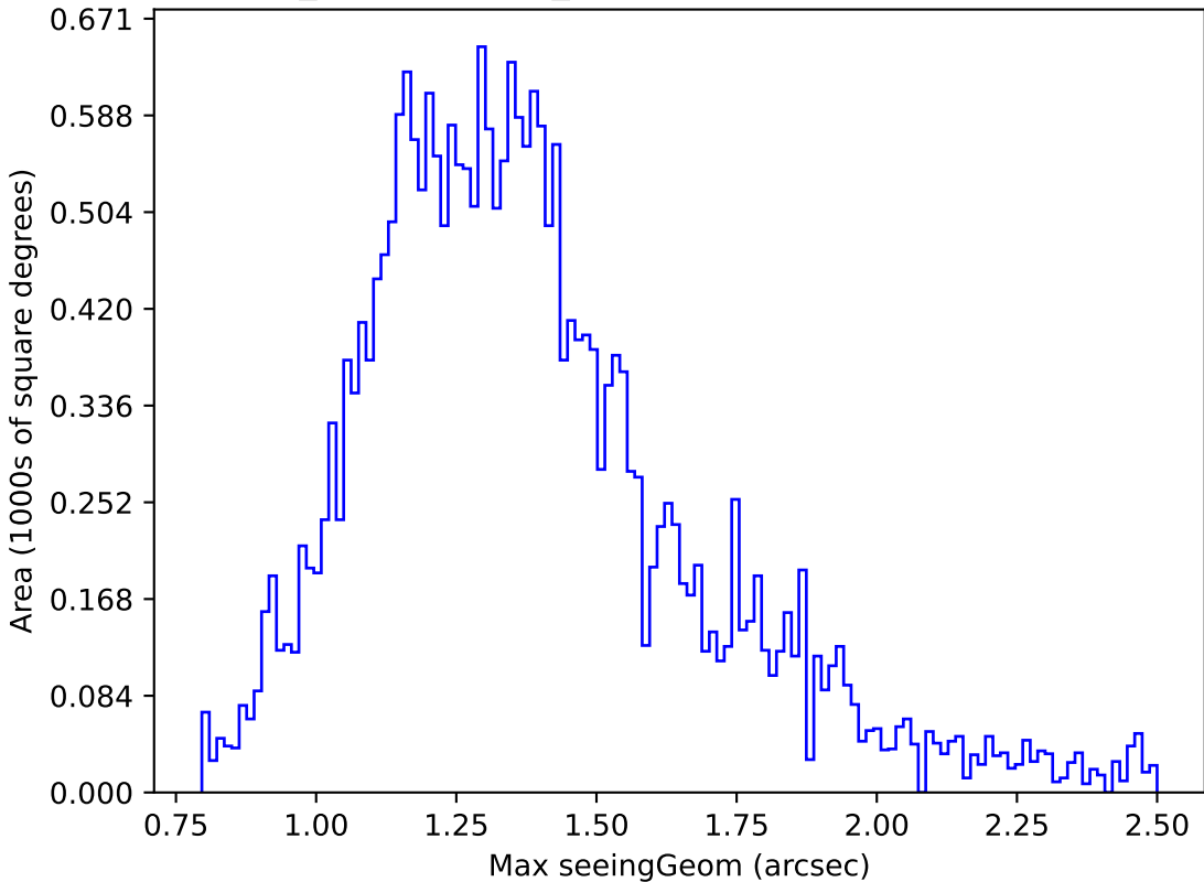
weather_cloudso1v3.4_10yrs Yr 1 r band: Max seeingGeom
