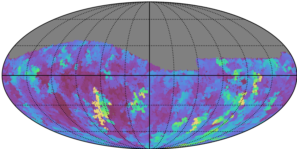
weather_cloudso1v3.4_10yrs Yr 1 g band: Max seeingGeom
