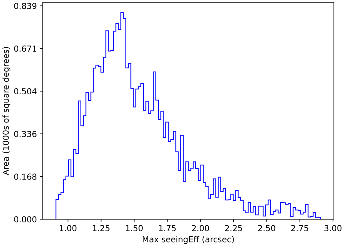
weather_cloudso1v3.4_10yrs Yr 1 z band: Max seeingEff
