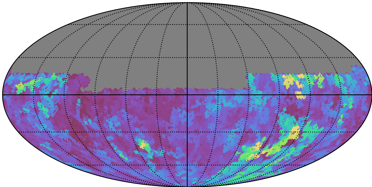
weather_cloudso1v3.4_10yrs Yr 1 u band: Max seeingEff
