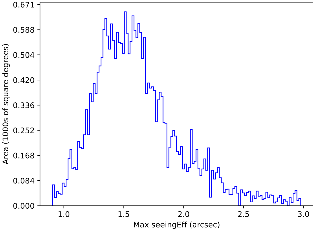
weather_cloudso1v3.4_10yrs Yr 1 r band: Max seeingEff
