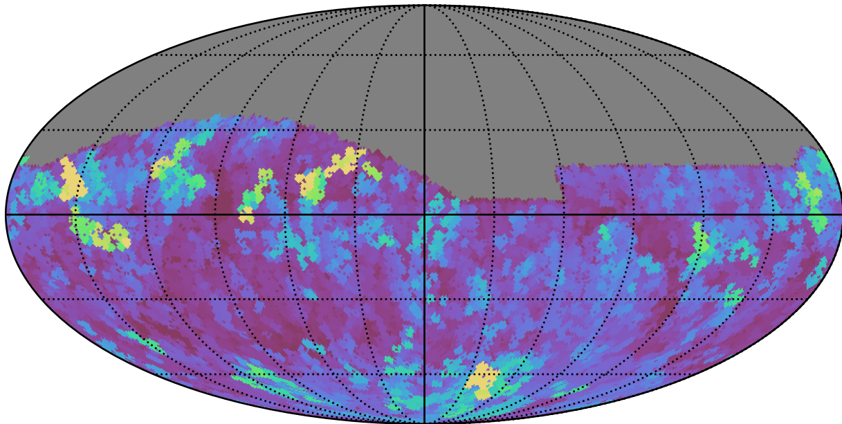
weather_cloudso1v3.4_10yrs Yr 1 i band: Max seeingEff
