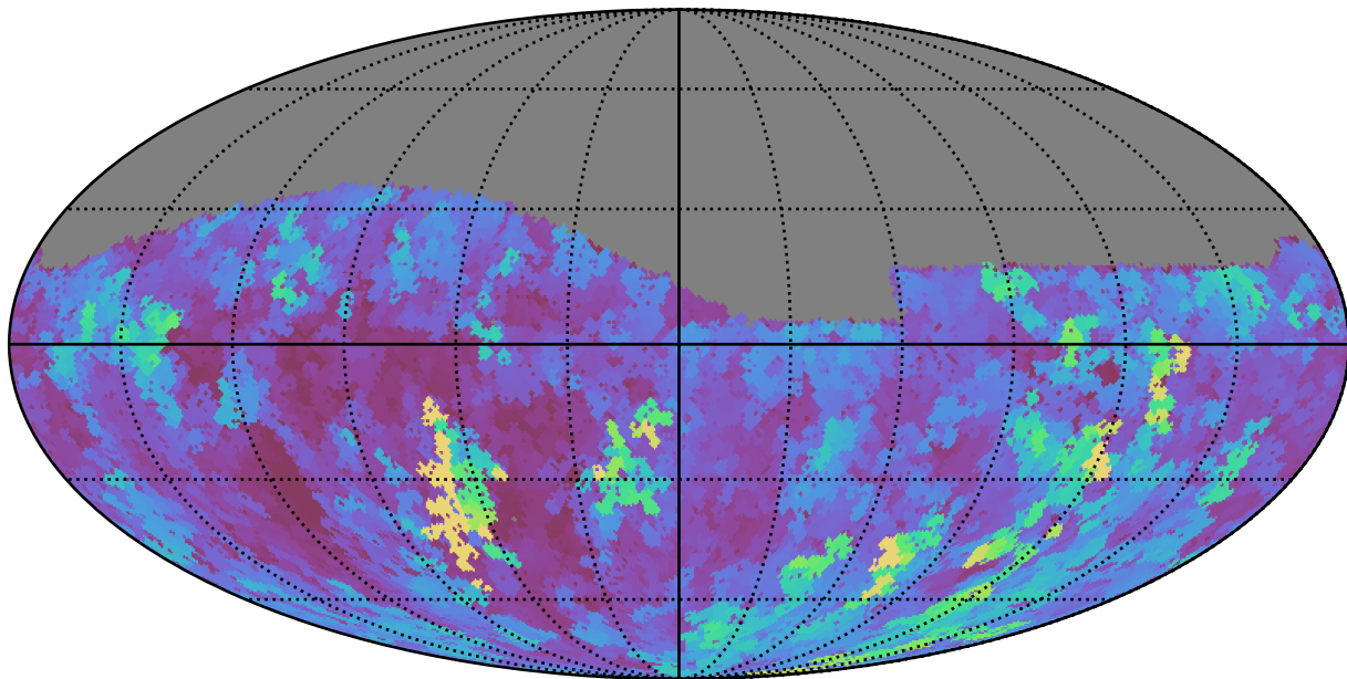
weather_cloudso1v3.4_10yrs Yr 1 g band: Max seeingEff
