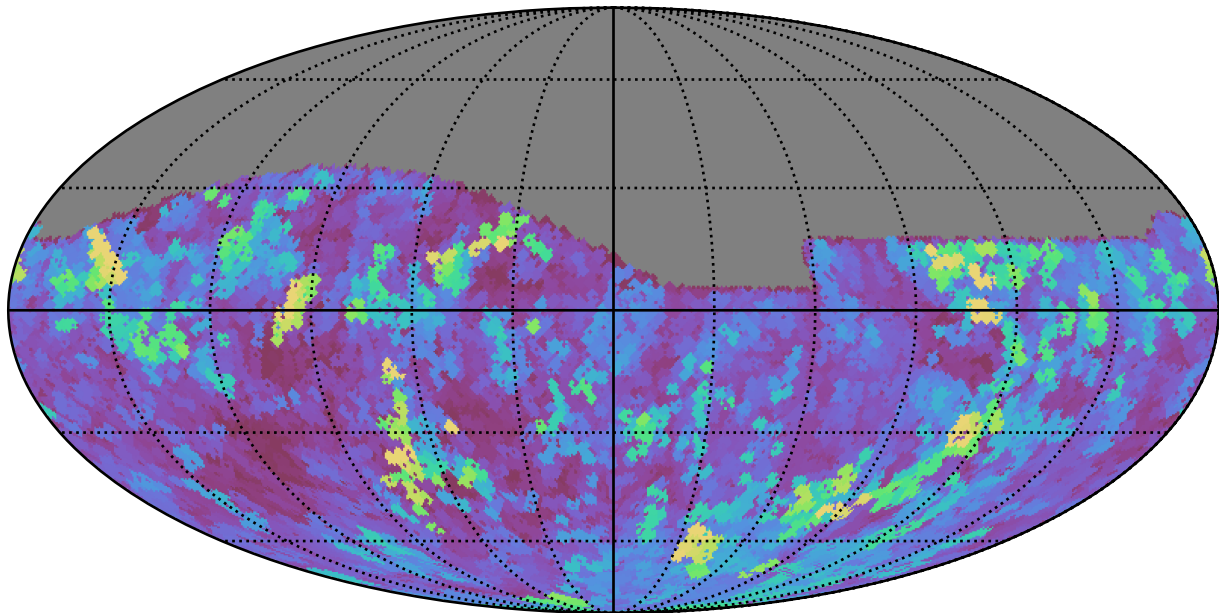
weather_cloudso1v3.4_10yrs Yr 1 all bands: Max seeingEff
