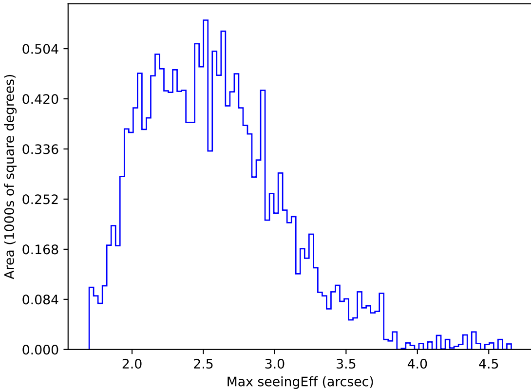
weather_cloudso1v3.4_10yrs WFD z band: Max seeingEff
