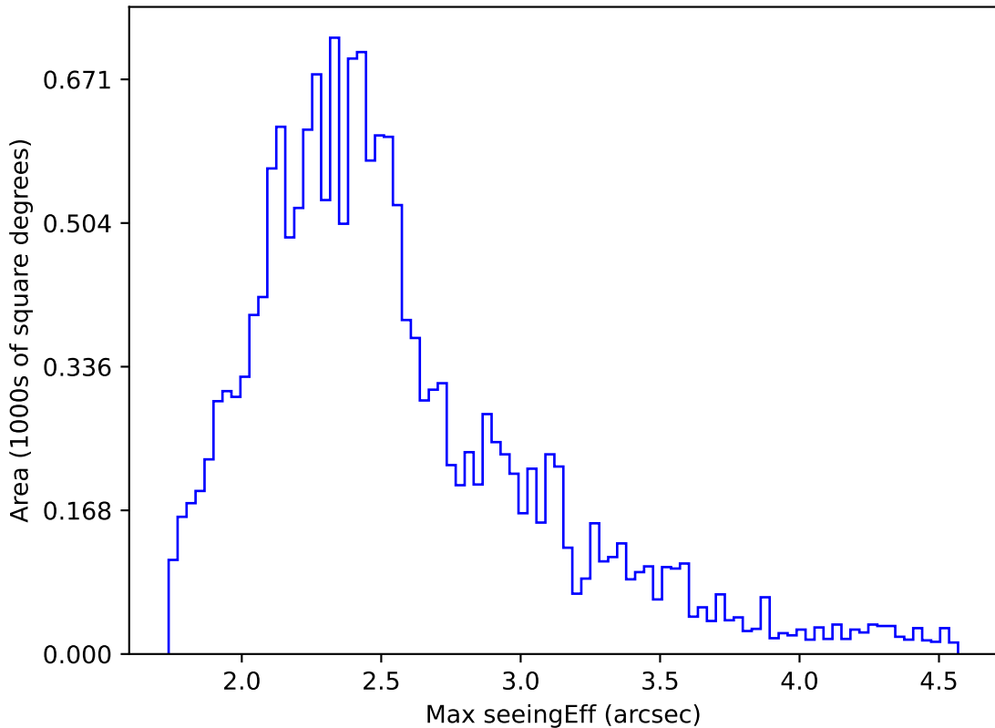
weather_cloudso1v3.4_10yrs WFD u band: Max seeingEff
