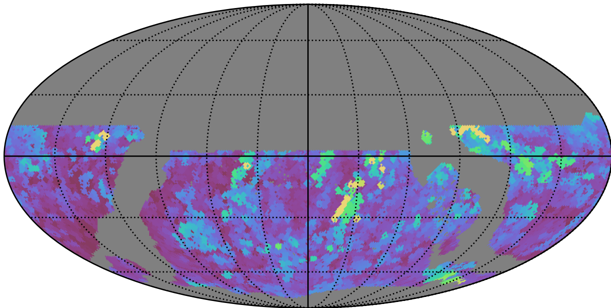
weather_cloudso1v3.4_10yrs WFD r band: Max seeingEff
