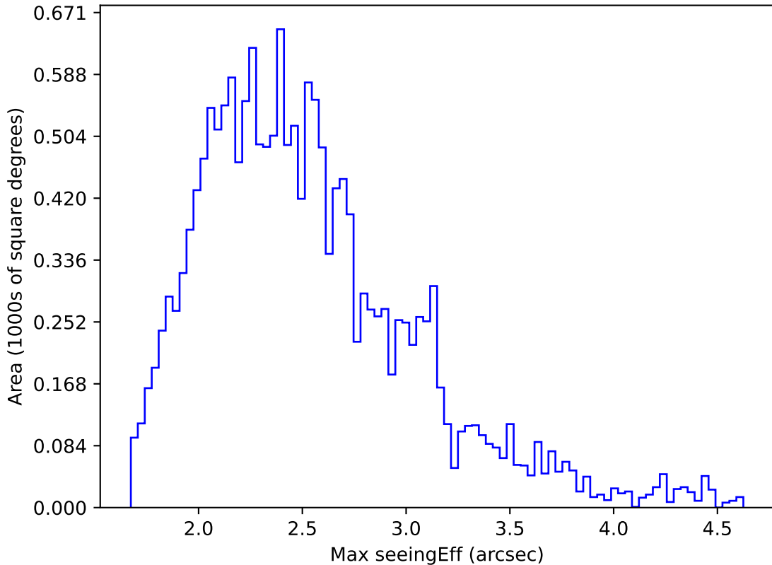
weather_cloudso1v3.4_10yrs WFD g band: Max seeingEff
