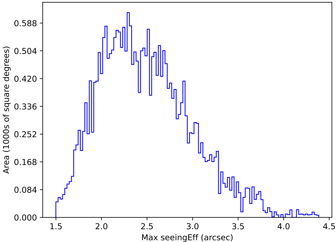
weather_cloudso1v3.4_10yrs All sky z band: Max seeingEff
