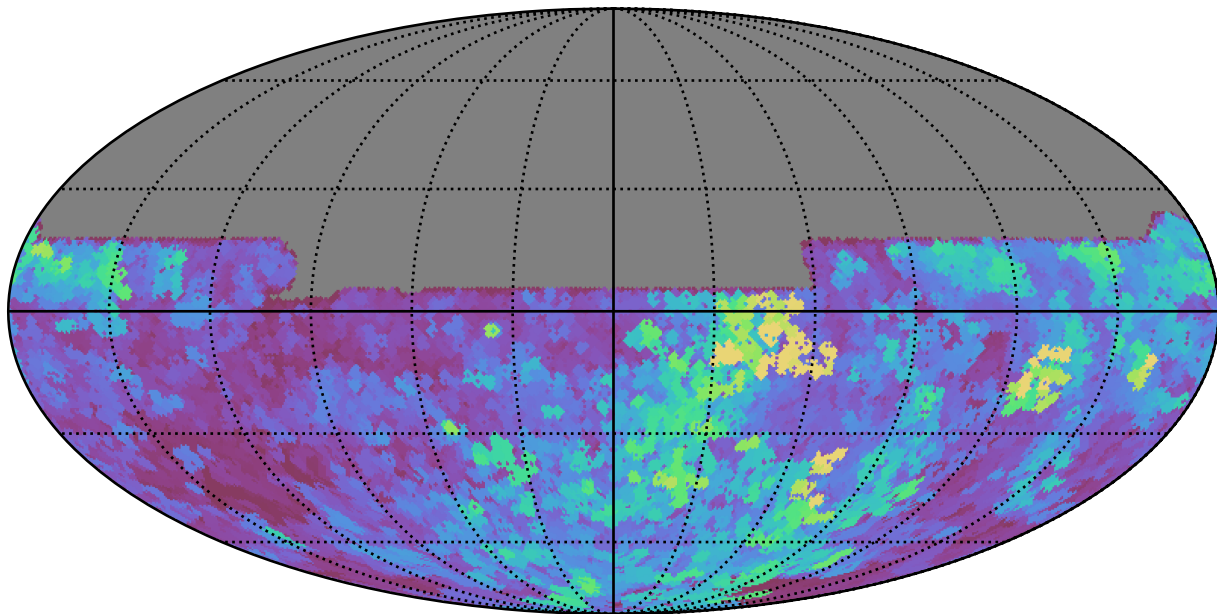
weather_cloudso1v3.4_10yrs All sky y band: Max seeingEff
