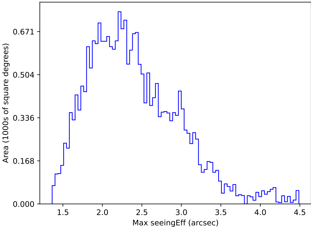
weather_cloudso1v3.4_10yrs All sky y band: Max seeingEff
