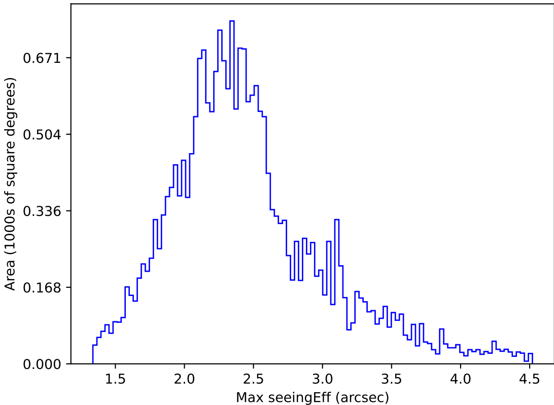
weather_cloudso1v3.4_10yrs All sky u band: Max seeingEff
