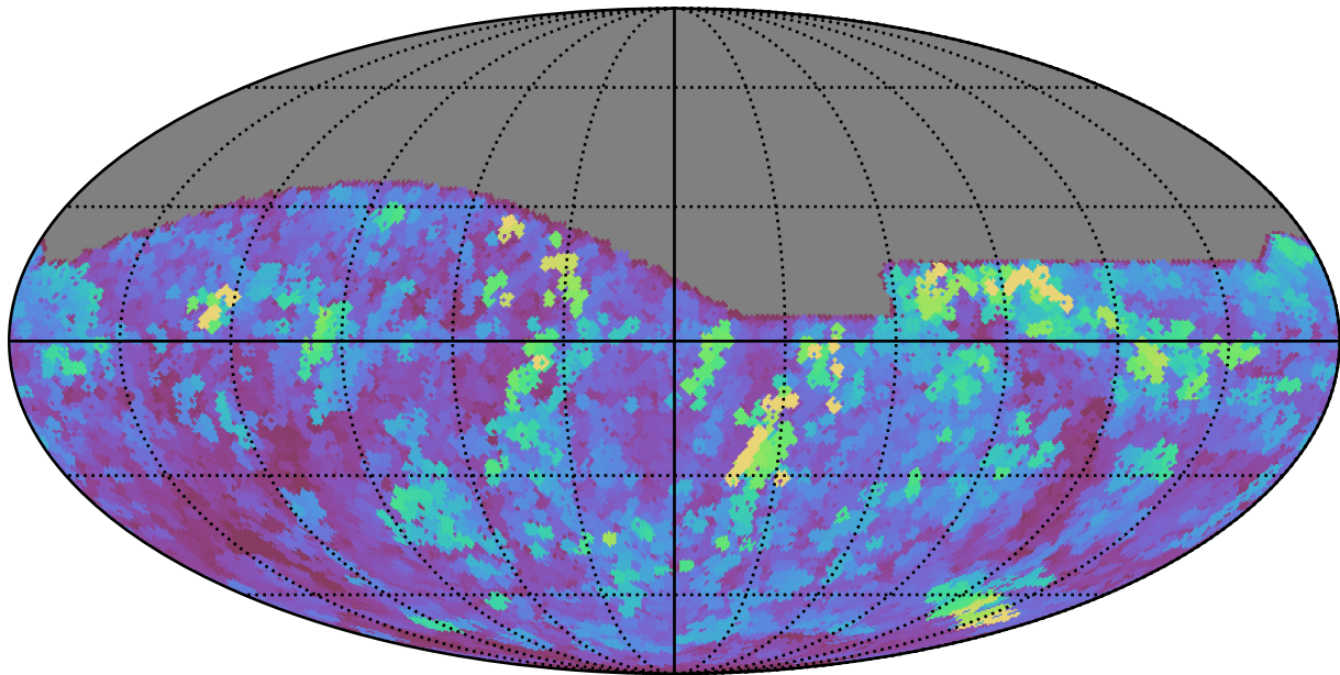
weather_cloudso1v3.4_10yrs All sky r band: Max seeingEff
