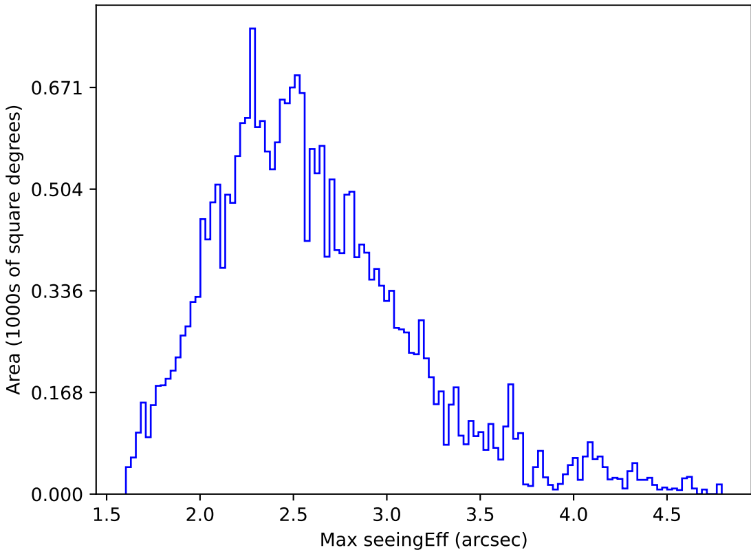
weather_cloudso1v3.4_10yrs All sky r band: Max seeingEff
