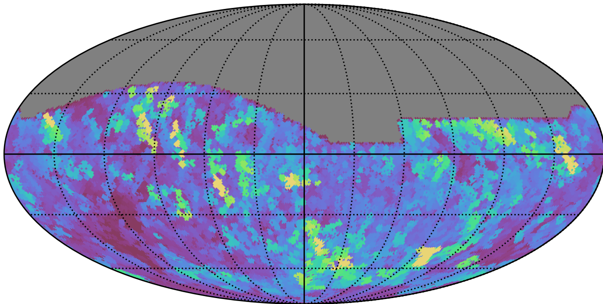
weather_cloudso1v3.4_10yrs All sky i band: Max seeingEff
