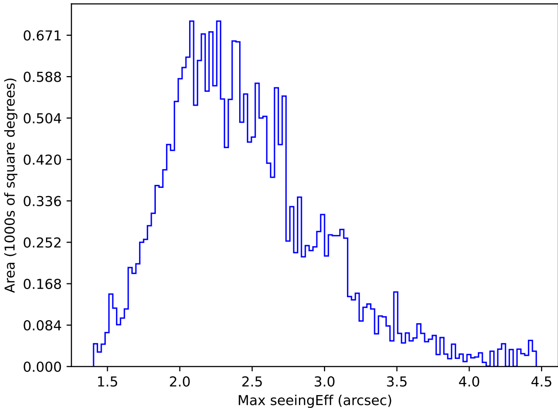
weather_cloudso1v3.4_10yrs All sky g band: Max seeingEff
