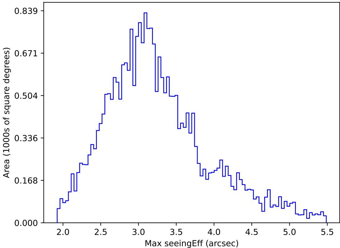
weather_cloudso1v3.4_10yrs All sky all bands: Max seeingEff
