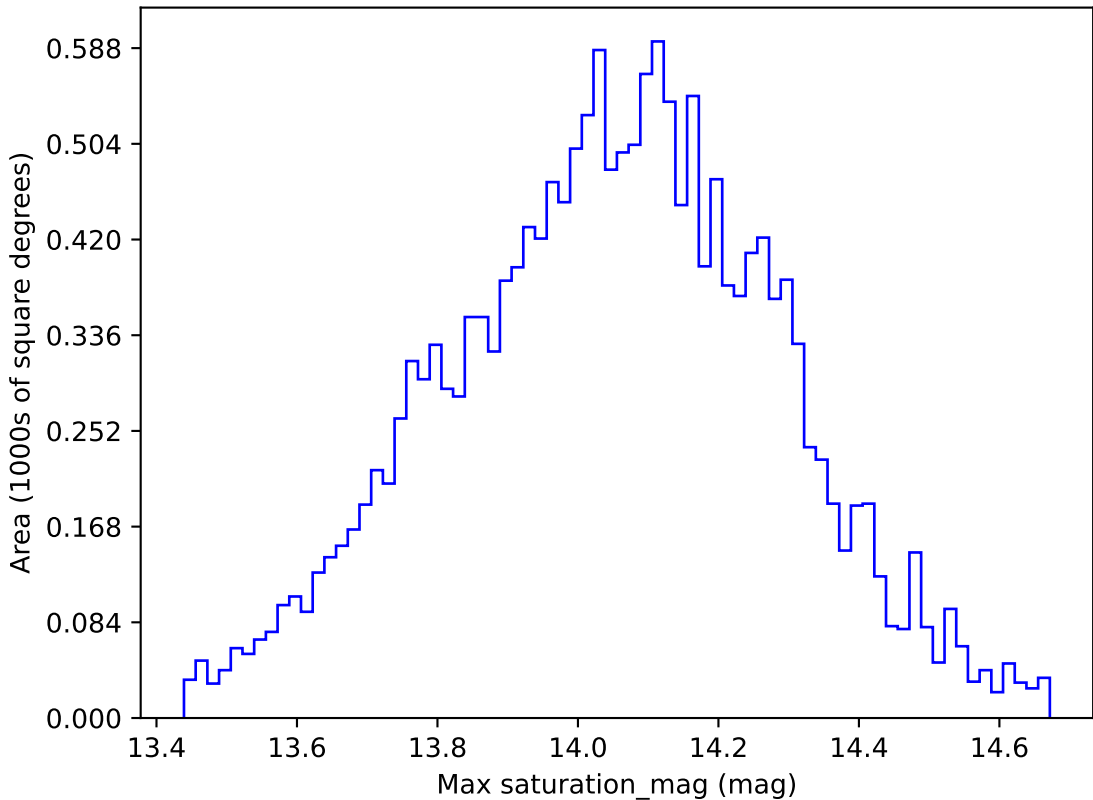
weather_cloudso1v3.4_10yrs WFD u band: Max saturation_mag
