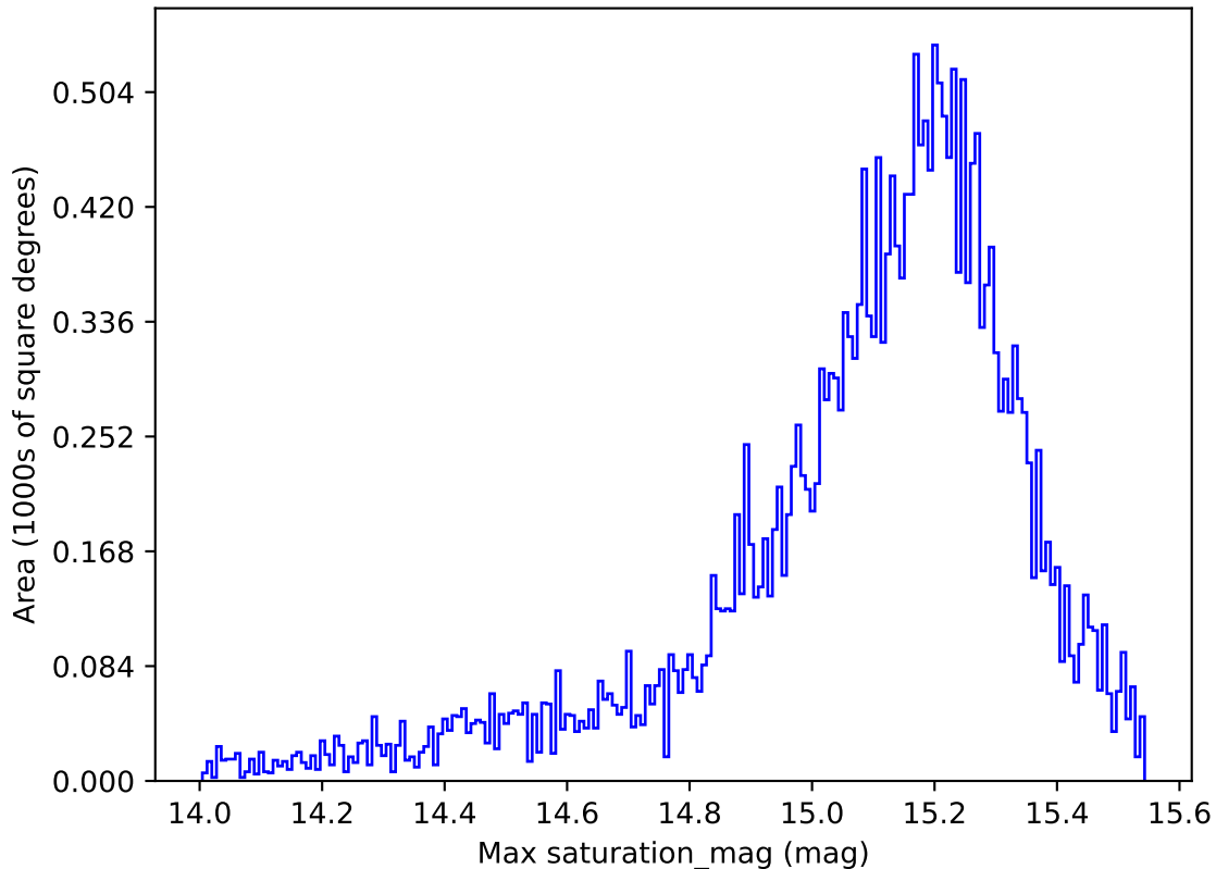
weather_cloudso1v3.4_10yrs All sky z band: Max saturation_mag
