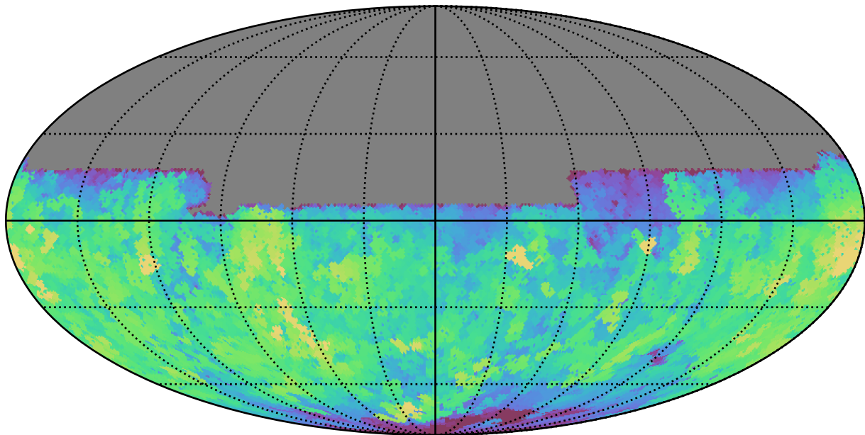
weather_cloudso1v3.4_10yrs All sky u band: Max saturation_mag
