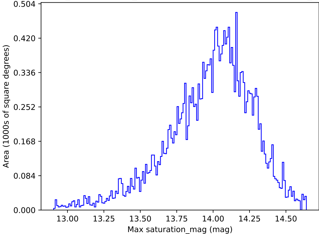
weather_cloudso1v3.4_10yrs All sky u band: Max saturation_mag
