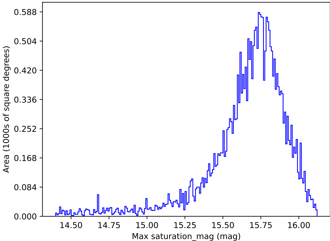
weather_cloudso1v3.4_10yrs All sky r band: Max saturation_mag
