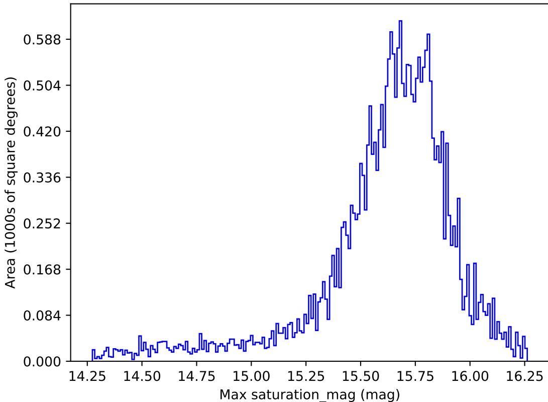
weather_cloudso1v3.4_10yrs All sky g band: Max saturation_mag
