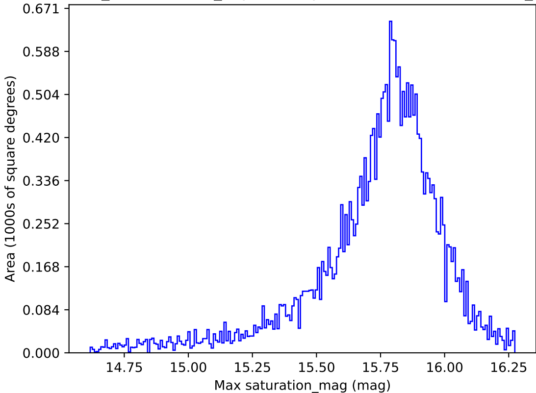
weather_cloudso1v3.4_10yrs All sky all bands: Max saturation_mag
