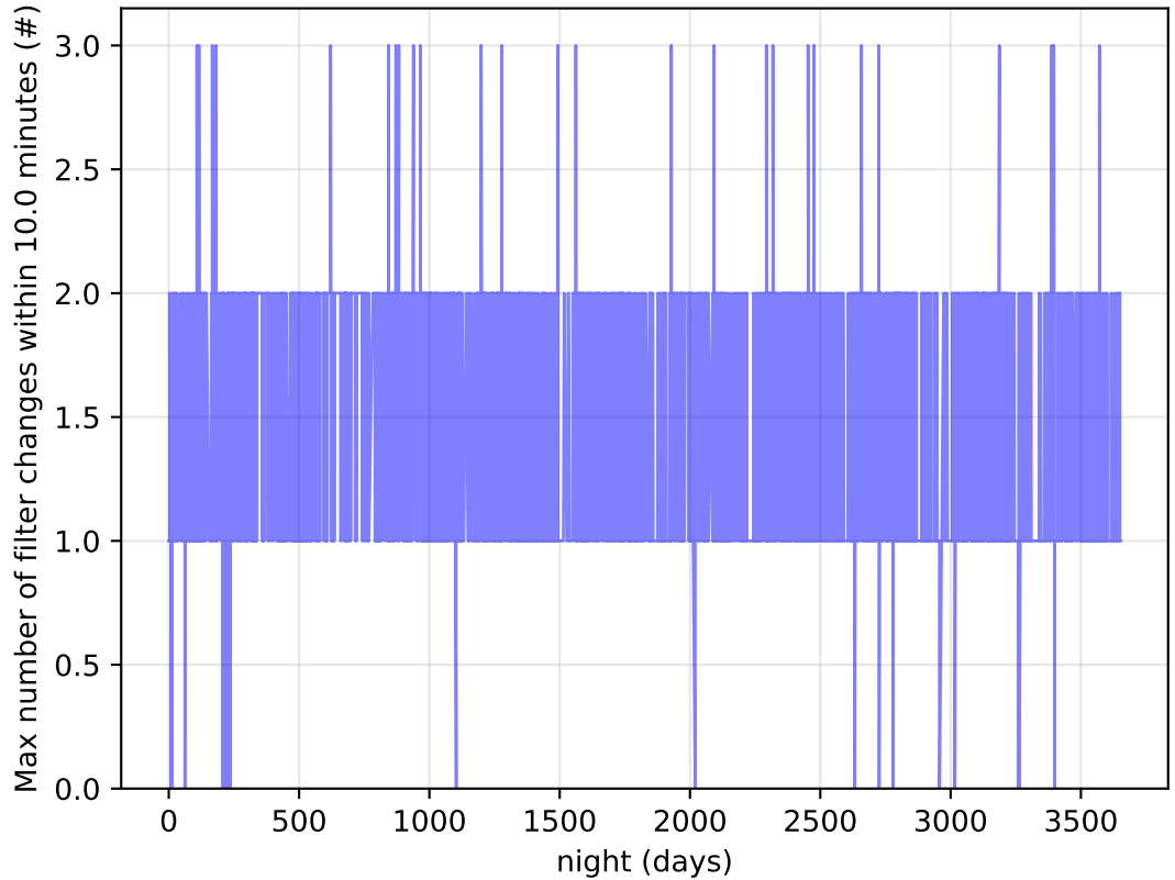
weather_cloudso1v3.4_10yrs Per Night: Max number of filter changes within 10.0 minutes
