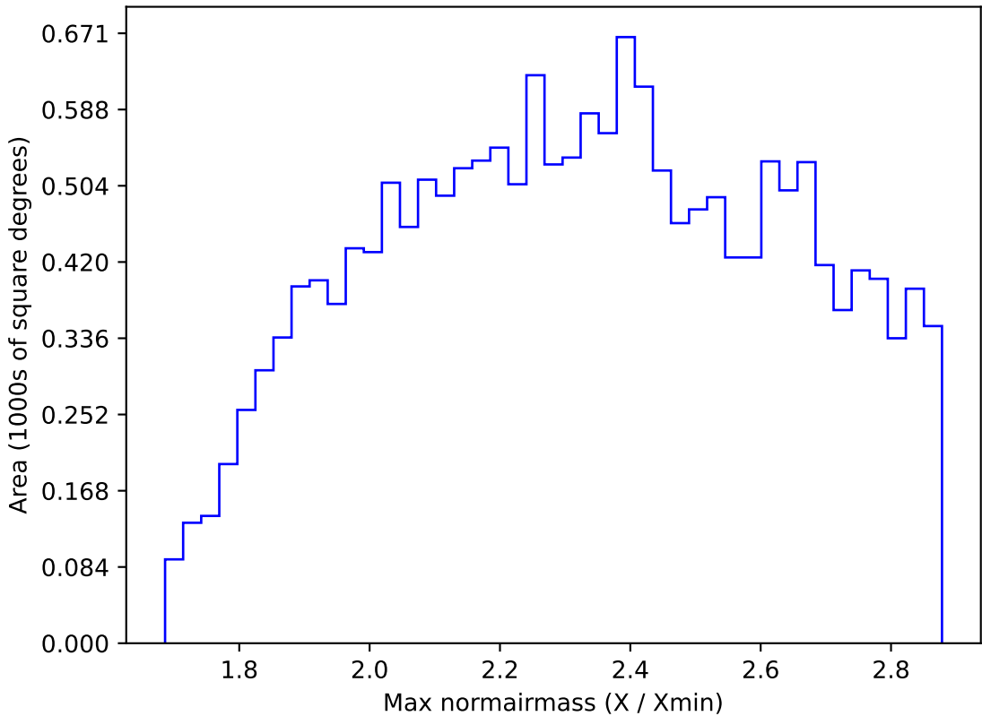
weather_cloudso1v3.4_10yrs WFD z band: Max normairmass
