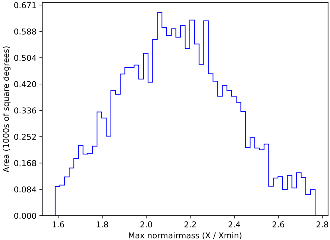
weather_cloudso1v3.4_10yrs WFD y band: Max normairmass
