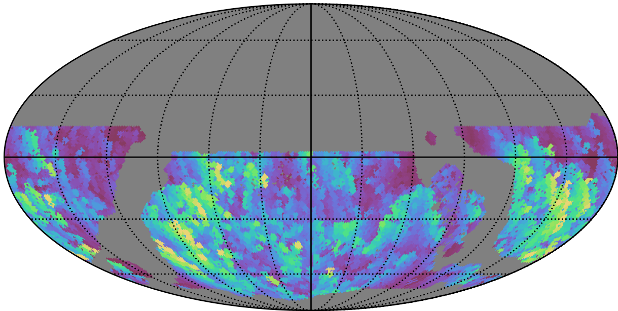
weather_cloudso1v3.4_10yrs WFD u band: Max normairmass
