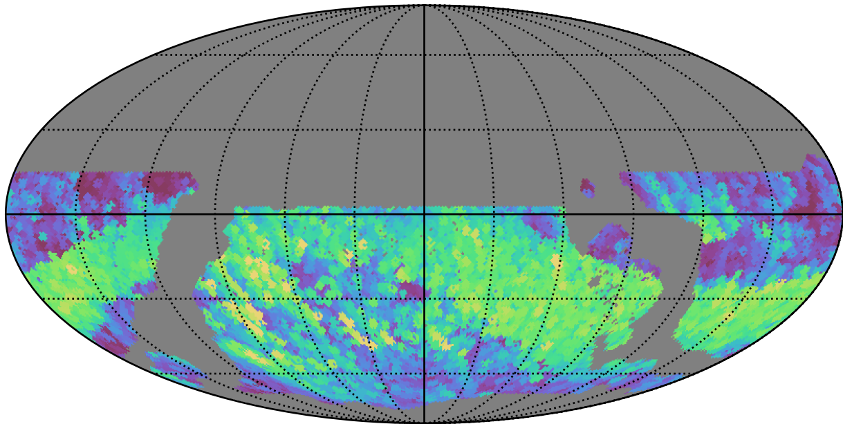
weather_cloudso1v3.4_10yrs WFD r band: Max normairmass
