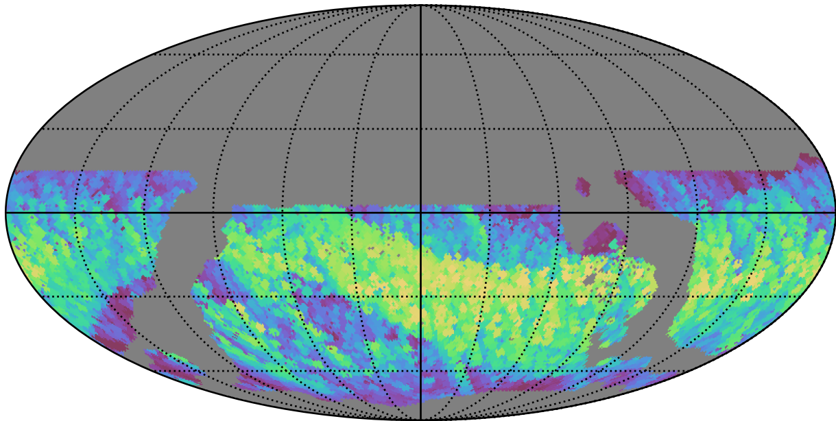
weather_cloudso1v3.4_10yrs WFD i band: Max normairmass
