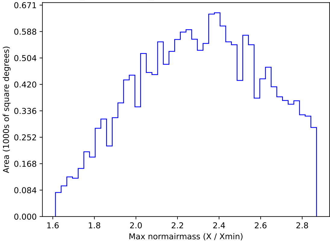
weather_cloudso1v3.4_10yrs WFD i band: Max normairmass
