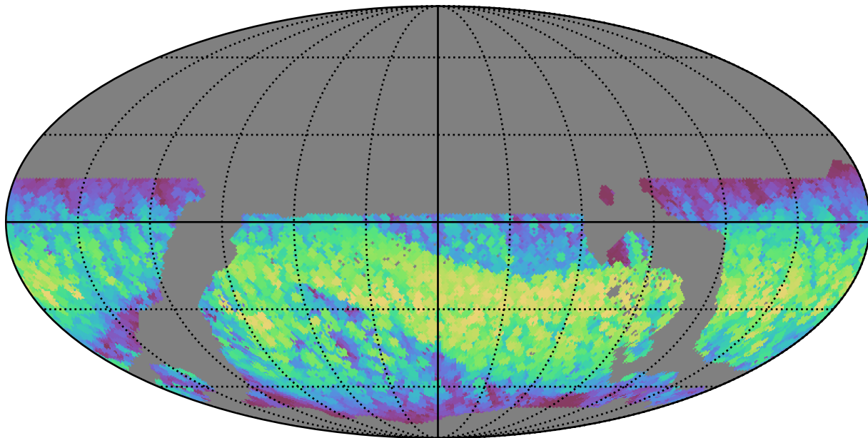
weather_cloudso1v3.4_10yrs WFD all bands: Max normairmass
