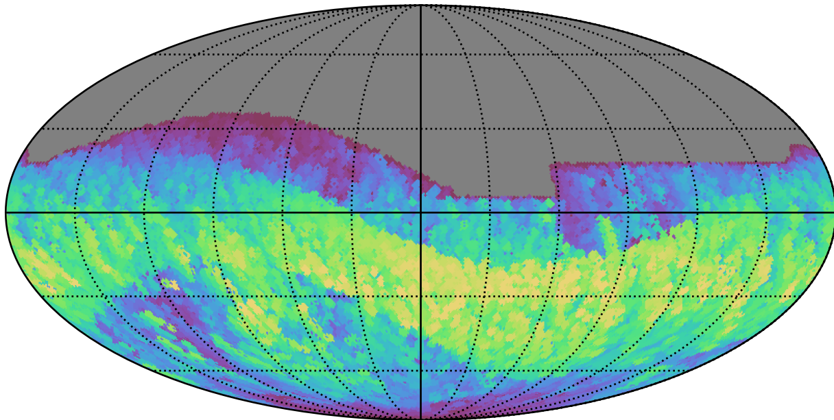
weather_cloudso1v3.4_10yrs All sky z band: Max normairmass
