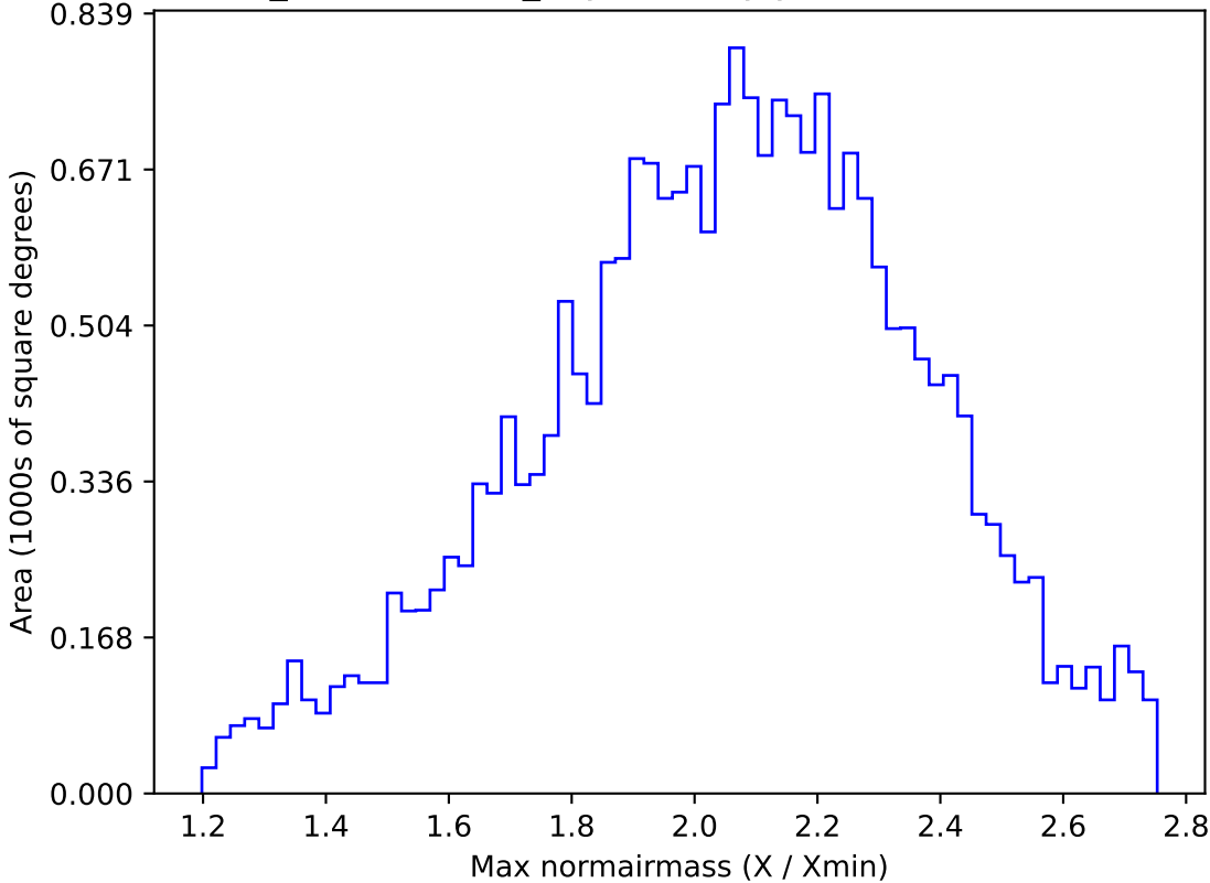
weather_cloudso1v3.4_10yrs All sky y band: Max normairmass
