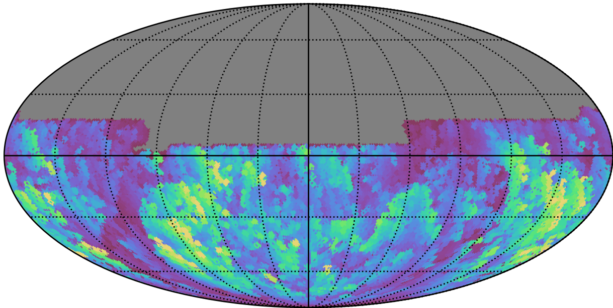
weather_cloudso1v3.4_10yrs All sky u band: Max normairmass
