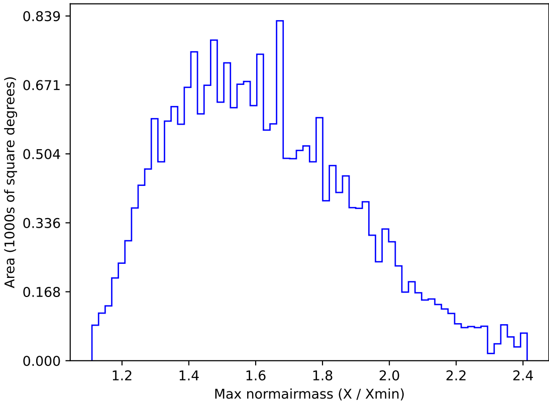
weather_cloudso1v3.4_10yrs All sky u band: Max normairmass
