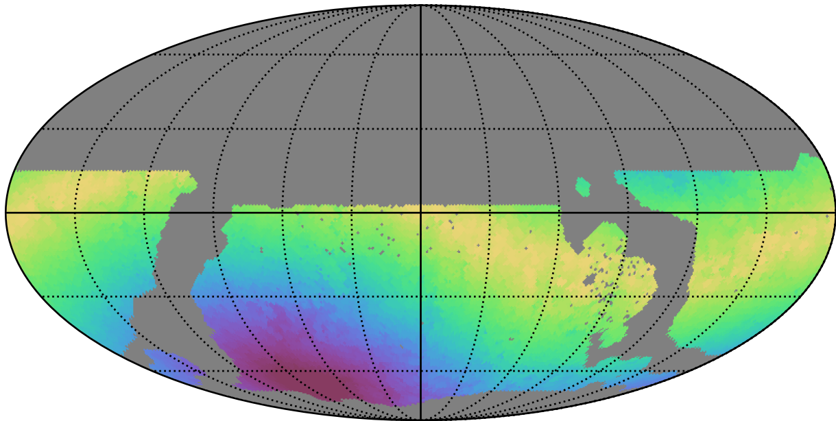
weather_cloudso1v3.4_10yrs WFD z band: Max moonDistance
