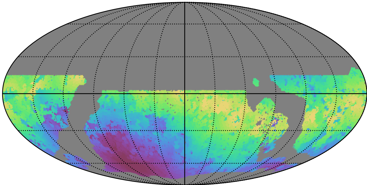
weather_cloudso1v3.4_10yrs WFD y band: Max moonDistance
