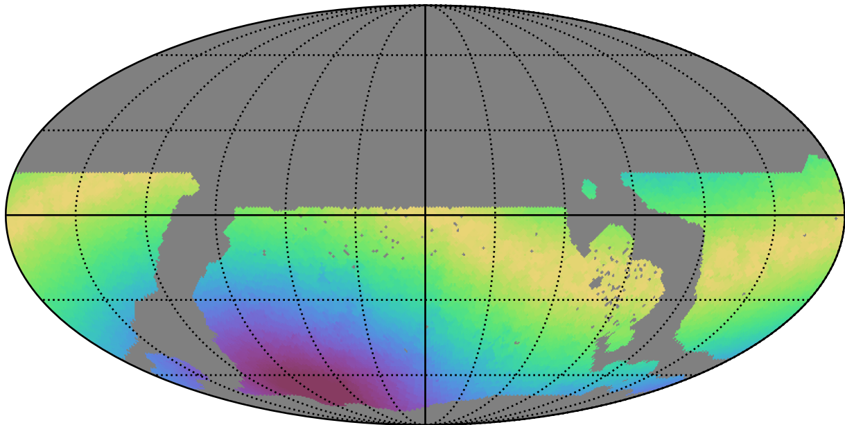
weather_cloudso1v3.4_10yrs WFD i band: Max moonDistance
