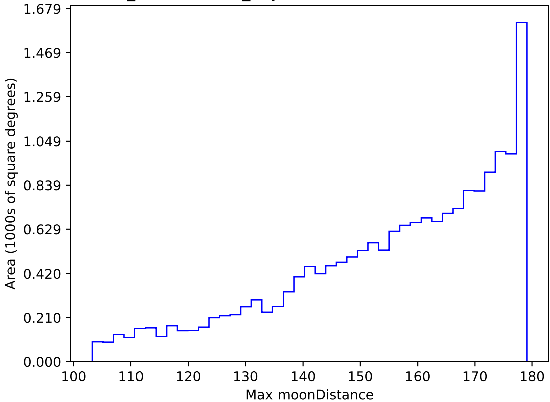
weather_cloudso1v3.4_10yrs WFD i band: Max moonDistance
