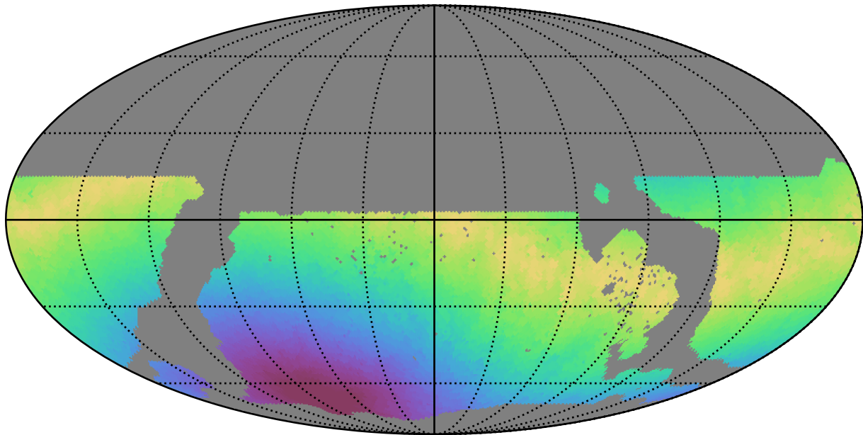
weather_cloudso1v3.4_10yrs WFD g band: Max moonDistance
