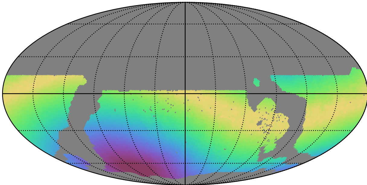
weather_cloudso1v3.4_10yrs WFD all bands: Max moonDistance
