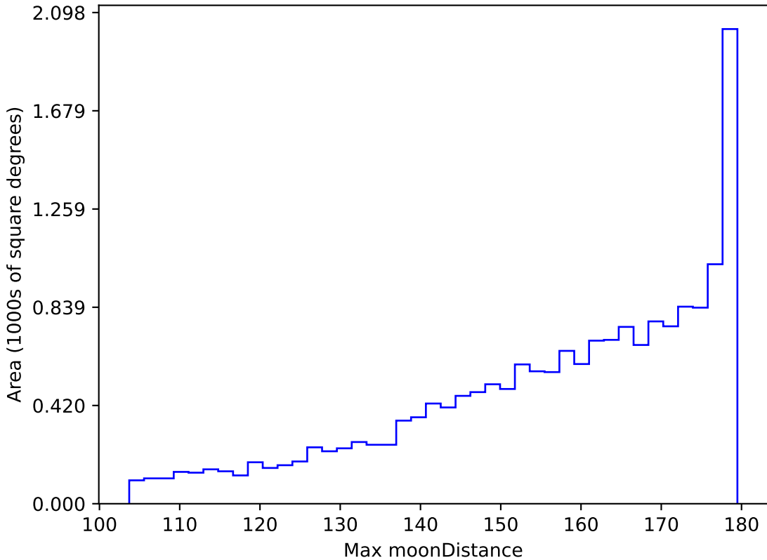
weather_cloudso1v3.4_10yrs WFD all bands: Max moonDistance
