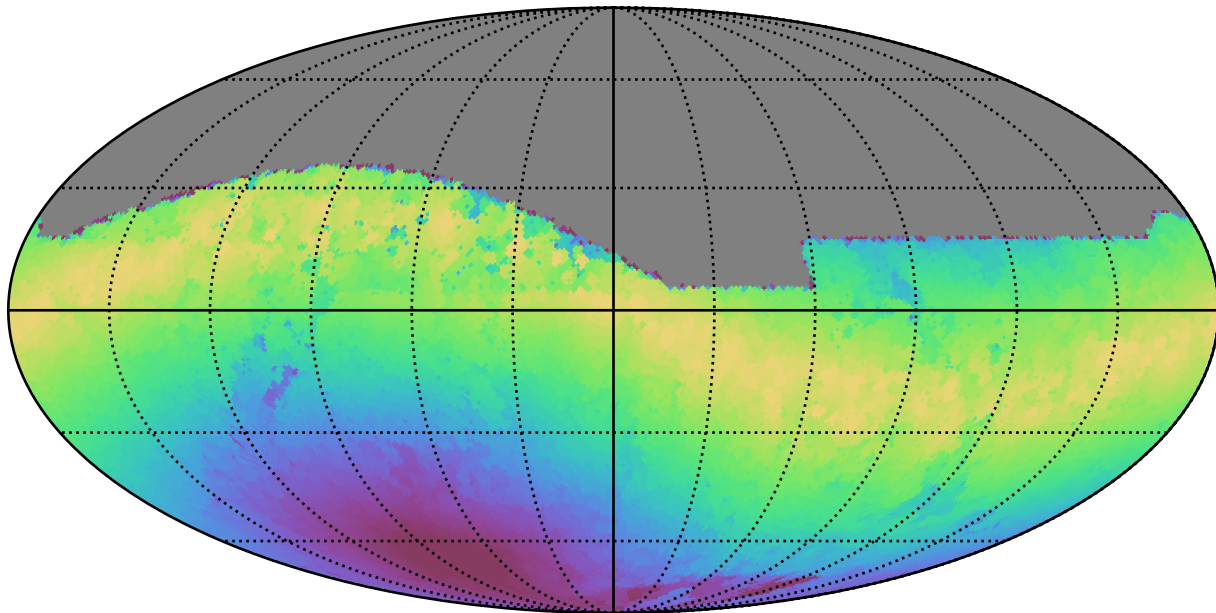
weather_cloudso1v3.4_10yrs All sky z band: Max moonDistance
