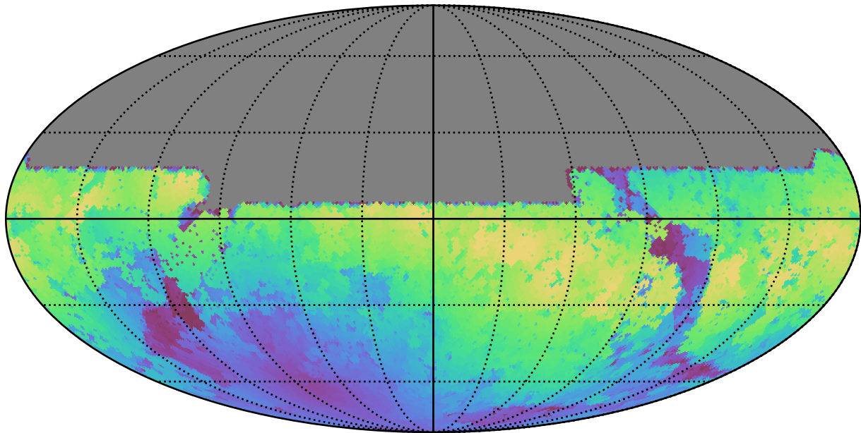
weather_cloudso1v3.4_10yrs All sky y band: Max moonDistance
