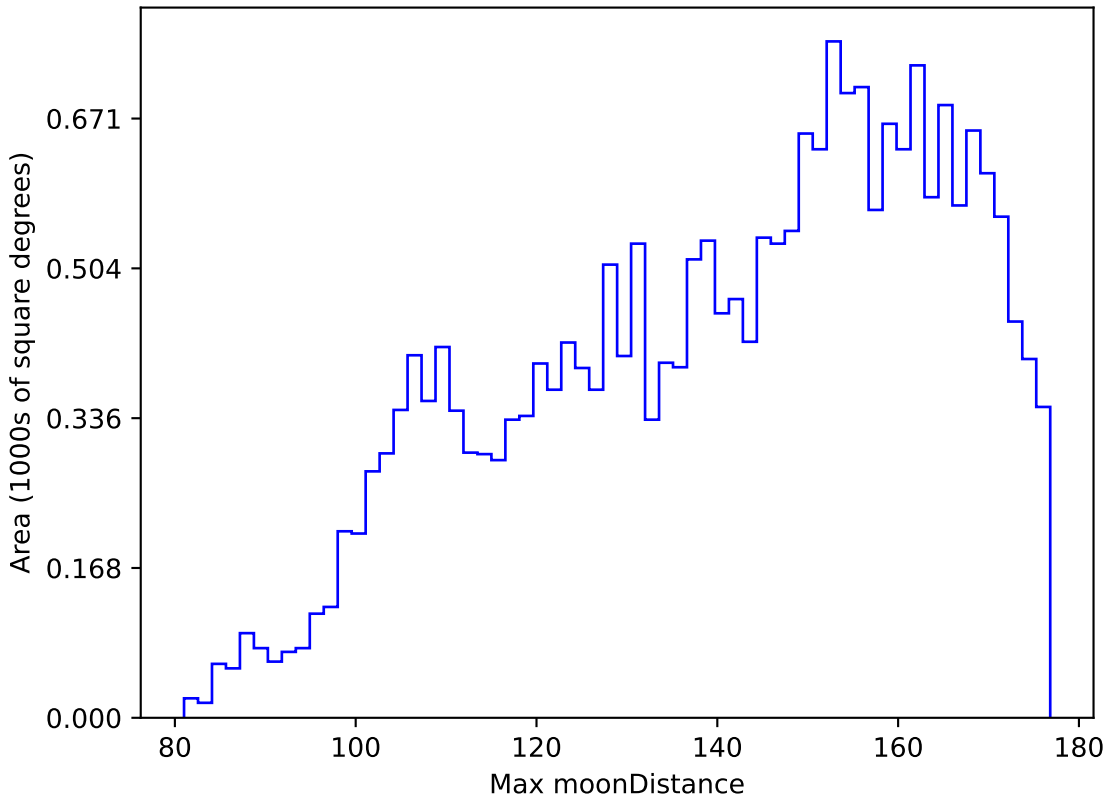
weather_cloudso1v3.4_10yrs All sky y band: Max moonDistance
